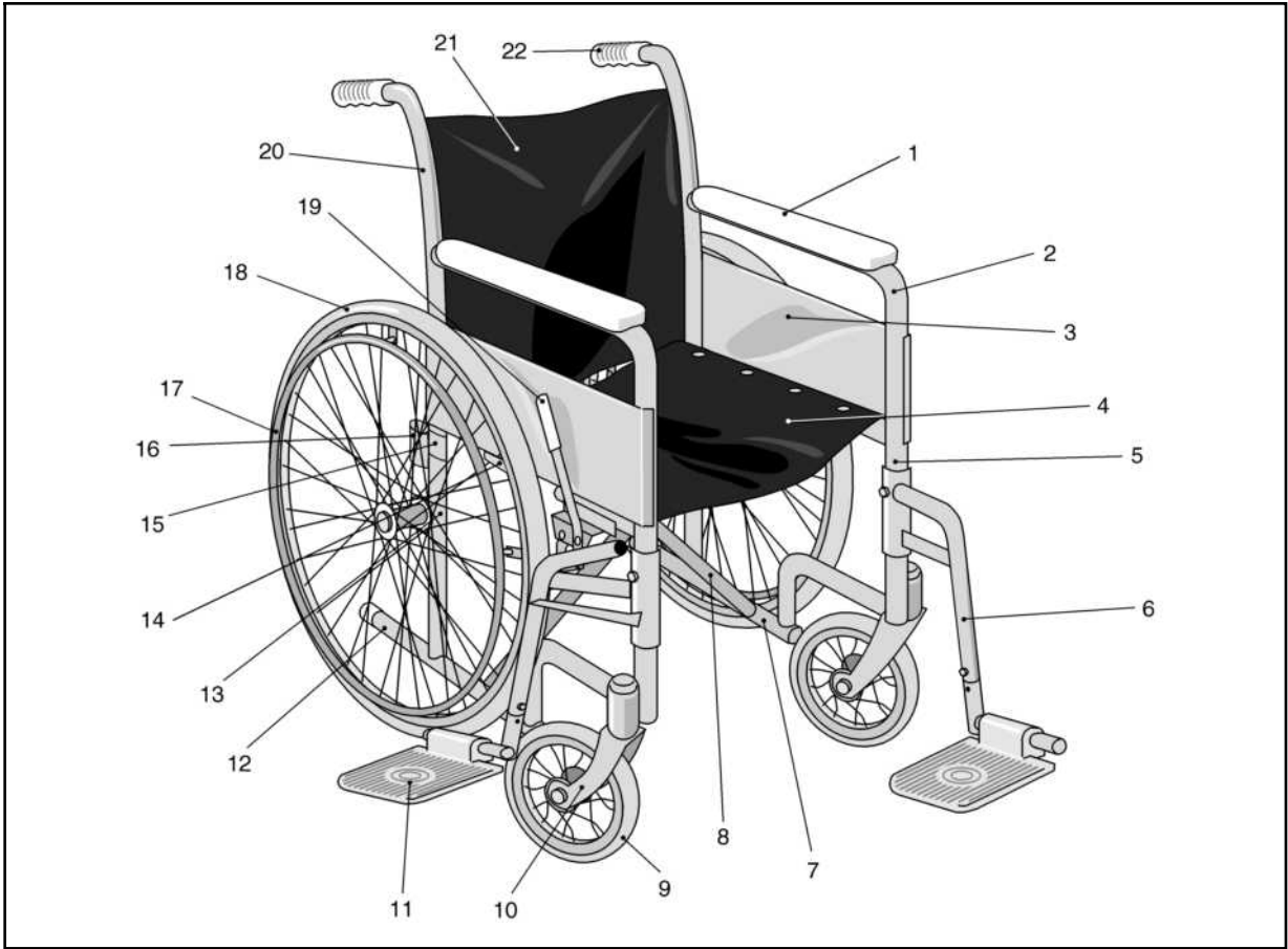
Figure 2 Wheelchair: 1. Arm pad; 2. Desk-style removable arm rest; 3. Clothes guard; 4. Sling seat; 5. Down tube; 6. Foot rest; 7. Bottom rail; 8. Cross-brace; 9. Caster; 10. Caster fork; 11. Footplate; 12. Tipping lever; 13. Axle; 14. Seat rail; 15. Arm rest bracket; 16. Arm rest bracket; 17. Handrim; 18. Wheel; 19. Wheel lock; 20. Back post; 21. Sling back; 22. Push handle
